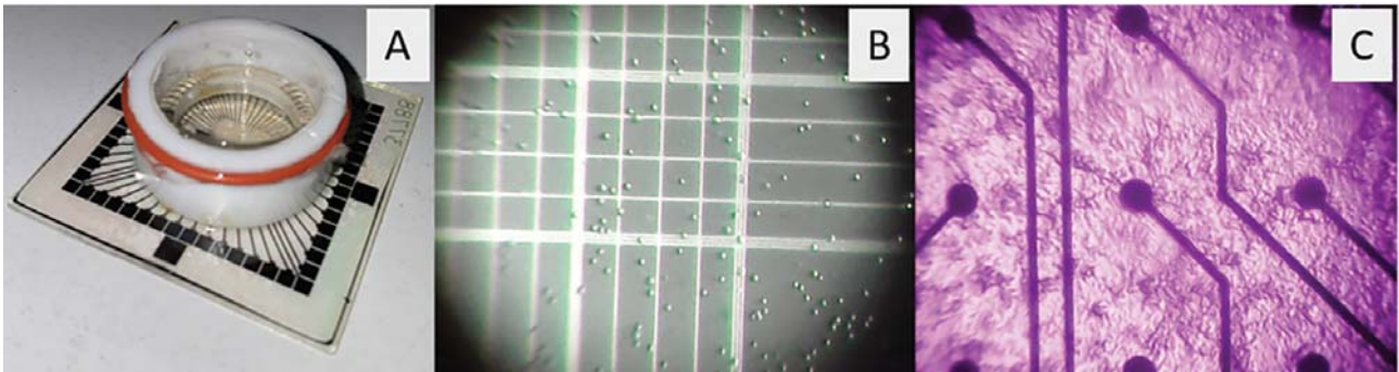
Fig. 1. A – Multielectrode array (MEA) with Teflon Millipore cover. B – DCC on the hemocytometer at 0 DIV, exhibiting adequate dispersion of about 25 healthy cells on 0.04 mm 2 (6250 cells in 1 \mu l) area. C – DCC attached to the MEA surface at the day 25 DIV, revealing developed neuronal network with axonal and dendritic fibers.
